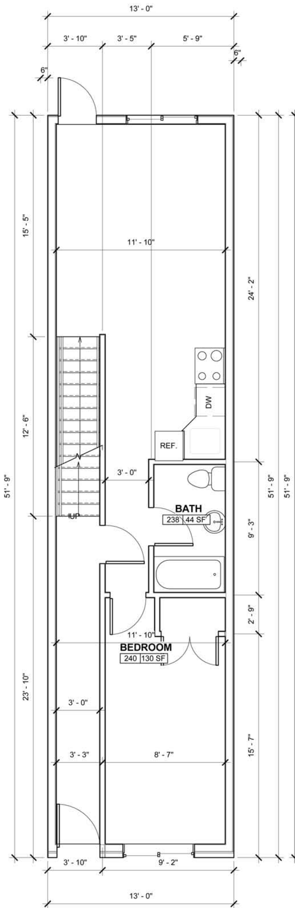
1st Floor
