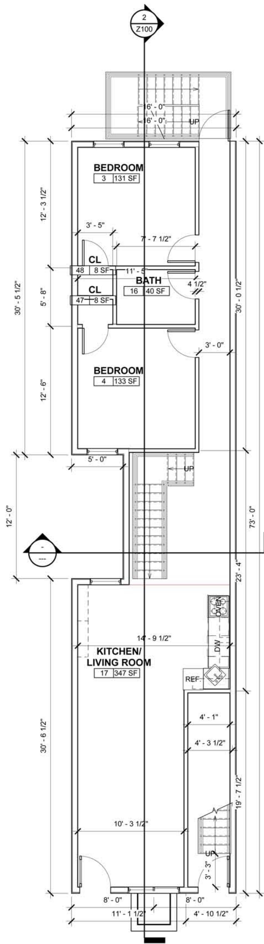
1st Floor
