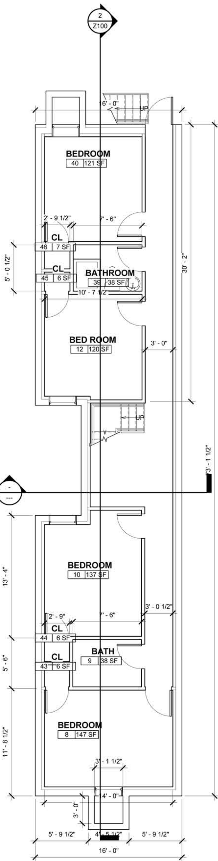
Ground Floor
