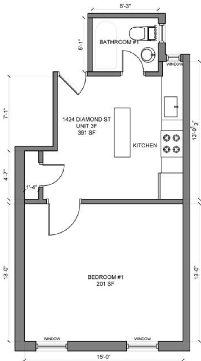
1424 DIAMOND ST EXISTING UNIT 3F
